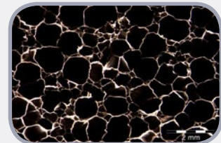
SH/Armaflex
